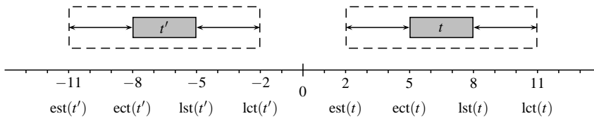
Fig. 1 Task t and its dual task t' using a minus view
